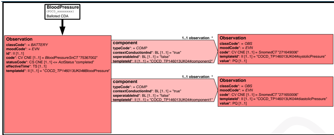
“Template” Representation (note this is a valid HL7 RMIM)
