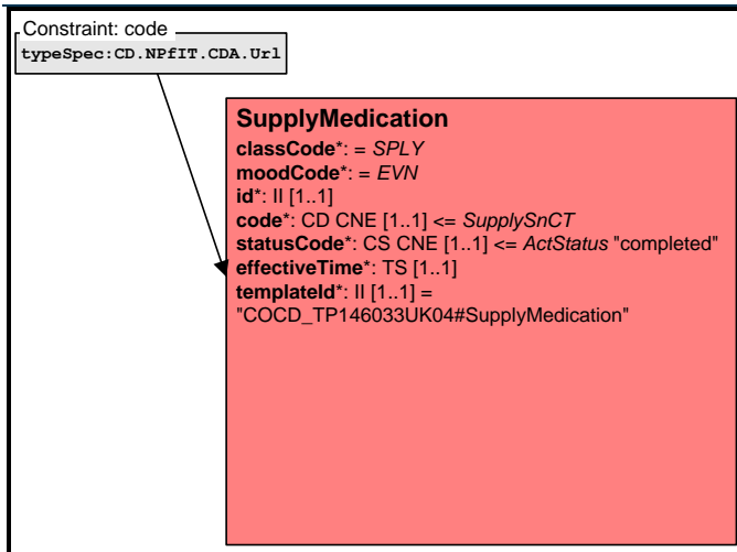
Constraint on CV
