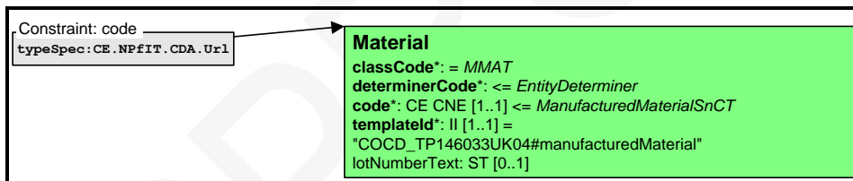
Constraint on CE
