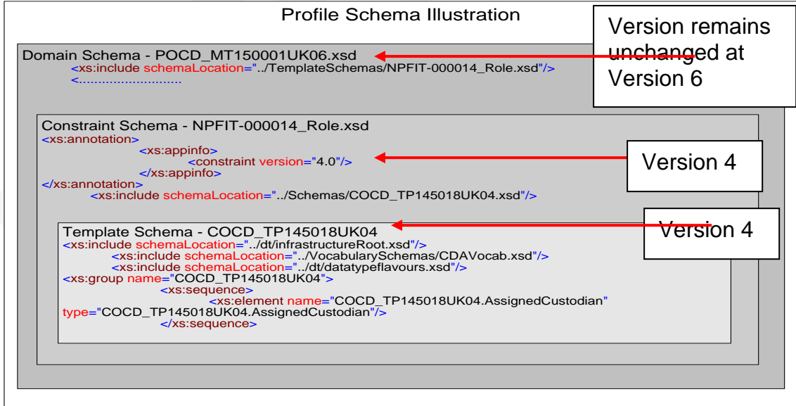
Illustration of up versioning within the profile schema collection when a template changes
